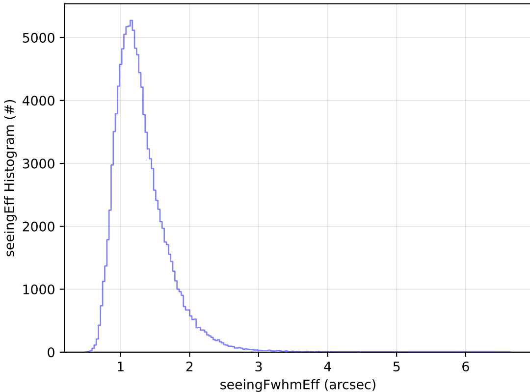
ddf_acor_sf15_lsf20_lsr20_v3.4_10yrs WFD u band: seeingEff Histogram
