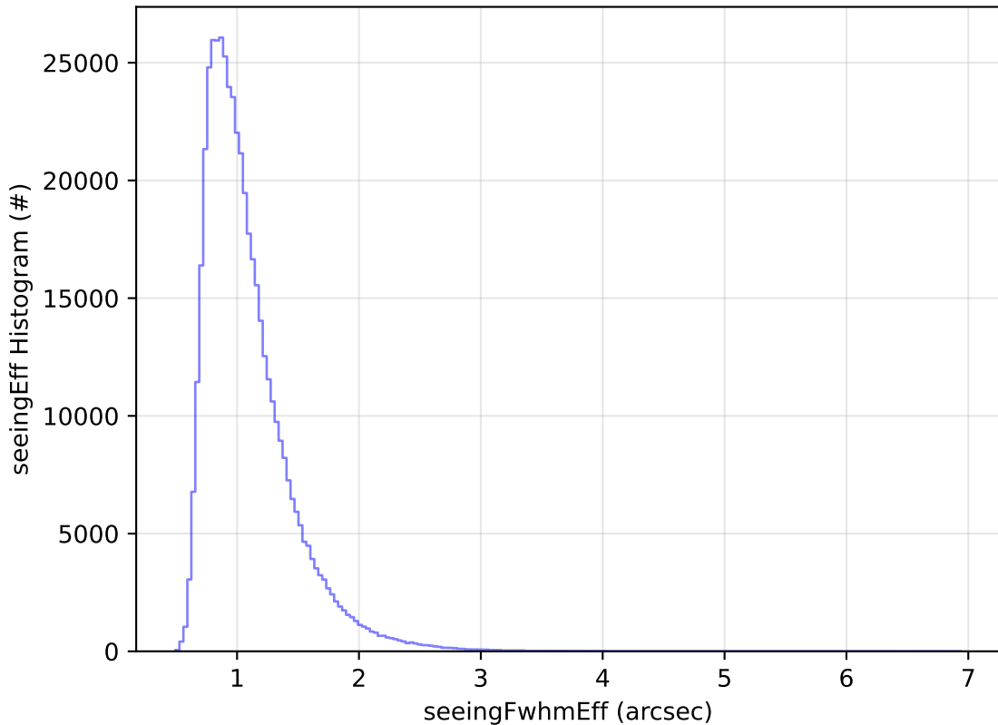
ddf_acor_sf15_lsf20_lsr20_v3.4_10yrs WFD i band: seeingEff Histogram
