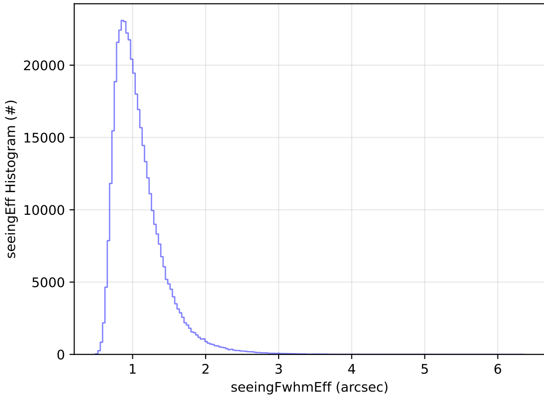
ddf_acor_sf15_lsf20_lsr20_v3.4_10yrs All sky z band: seeingEff Histogram
