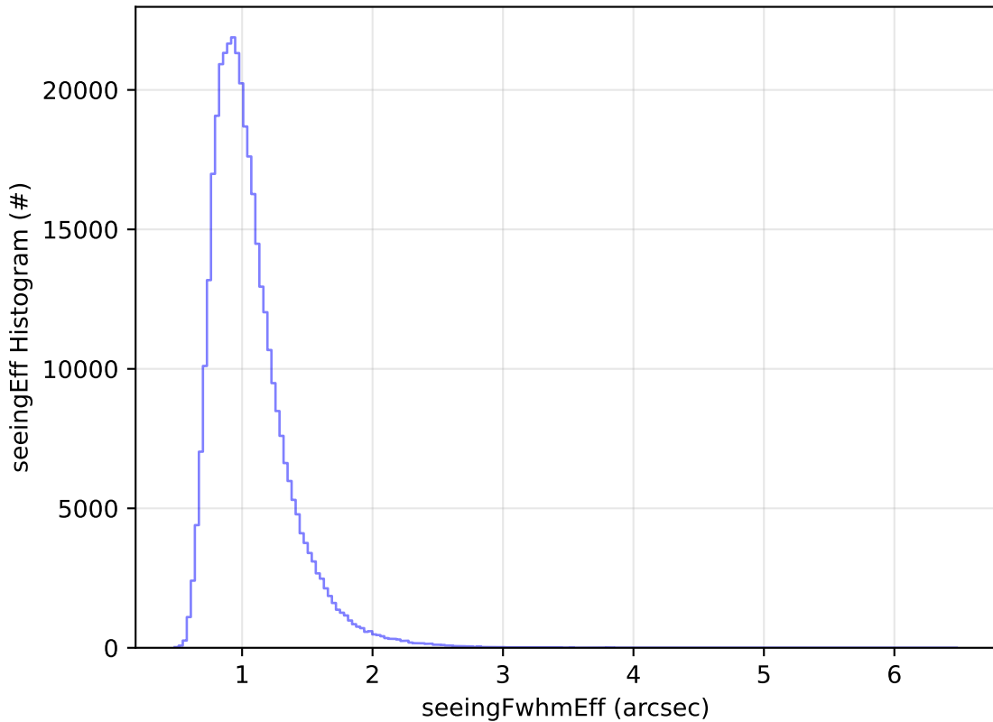
ddf_acor_sf15_lsf20_lsr20_v3.4_10yrs All sky y band: seeingEff Histogram
