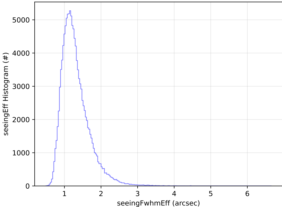
ddf_acor_sf15_ls20_lsr20_v3.4_10yrs All sky u band: seeingEff Histogram
