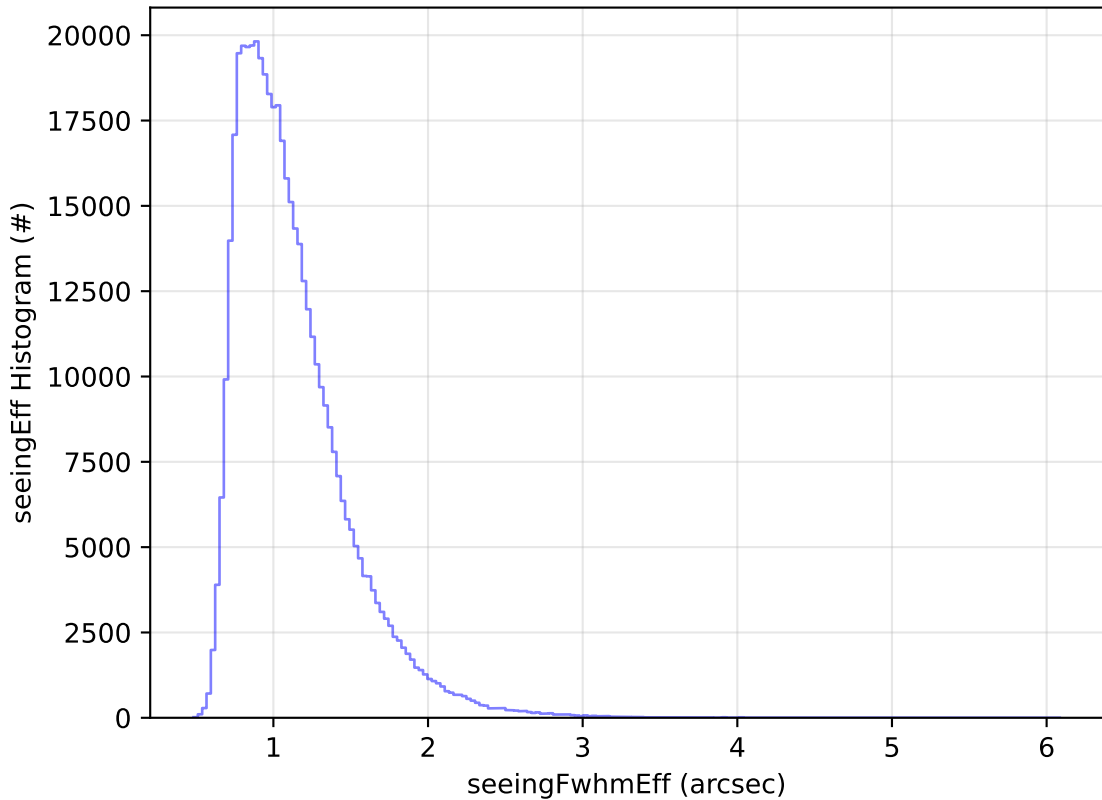
ddf_acor_sf15_lsf20_lsr20_v3.4_10yrs All sky r band: seeingEff Histogram
