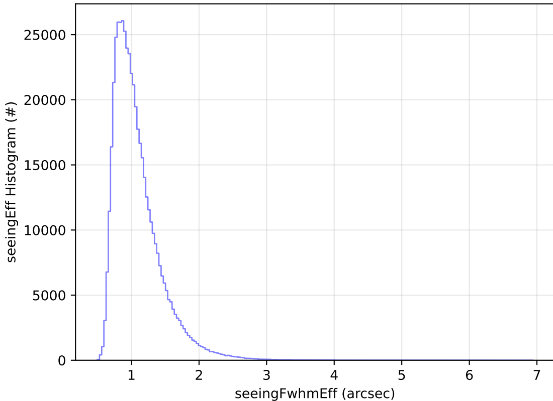
ddf_acor_sf15_lsf20_lsr20_v3.4_10yrs All sky i band: seeingEff Histogram
