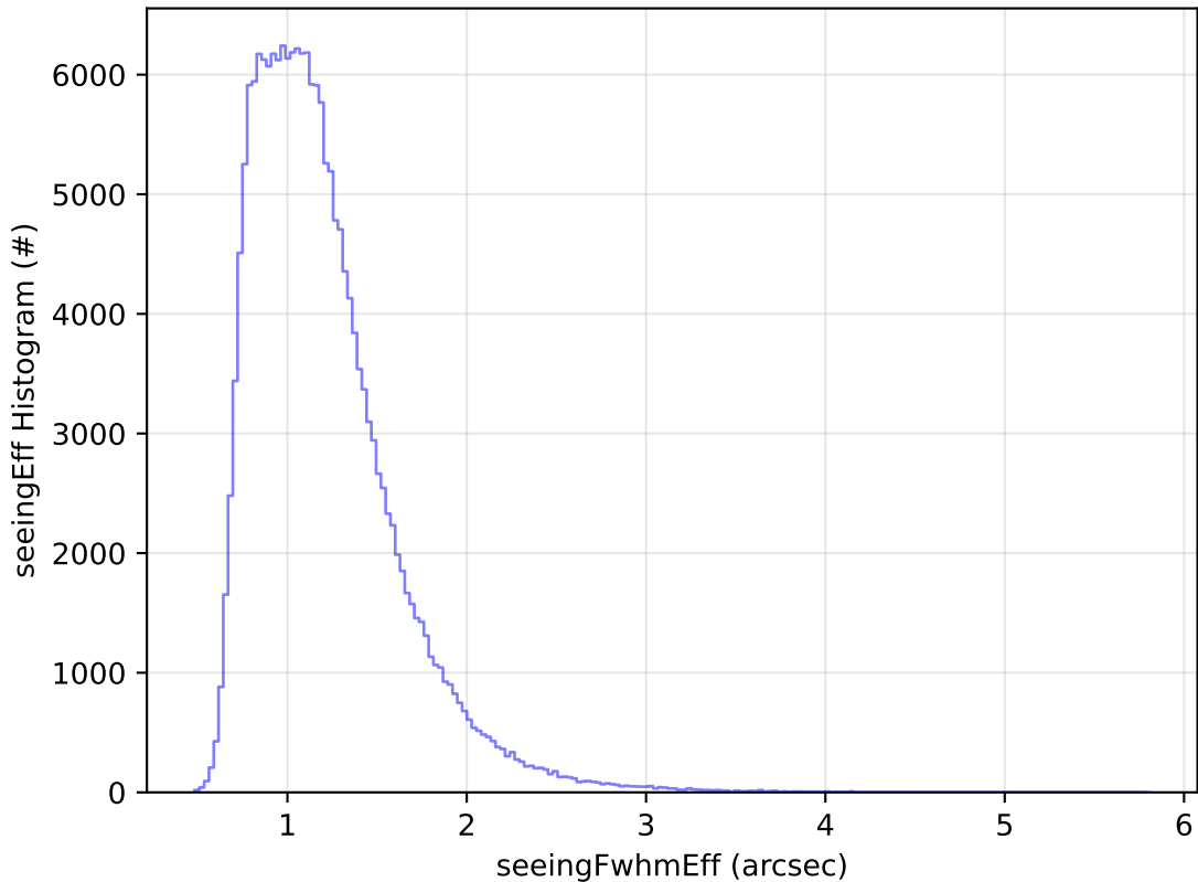
ddf_acor_sf15_lsf20_lsr20_v3.4_10yrs All sky g band: seeingEff Histogram
