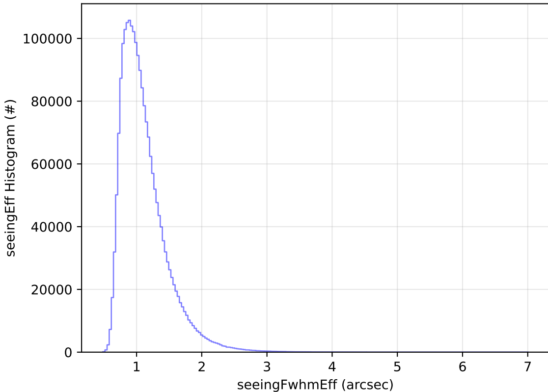
ddf_acor_sf15_lsf20_lsr20_v3.4_10yrs All sky all bands: seeingEff Histogram
