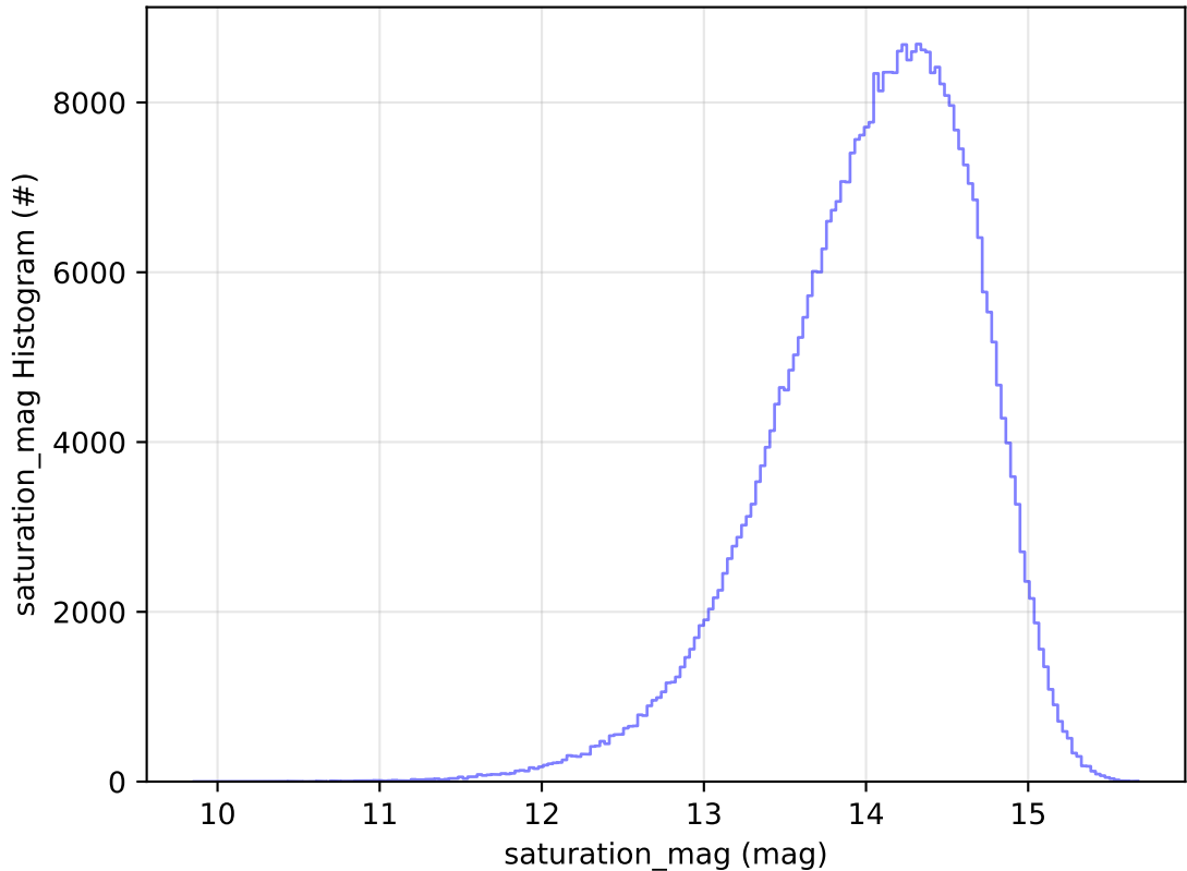
ddf_acor_sf15_lsf20_lsr20_v3.4_10yrs WFD z band: saturation_mag Histogram
