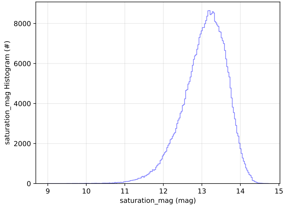
ddf_acor_sf15_lsf20_lsr20_v3.4_10yrs WFD y band: saturation_mag Histogram
