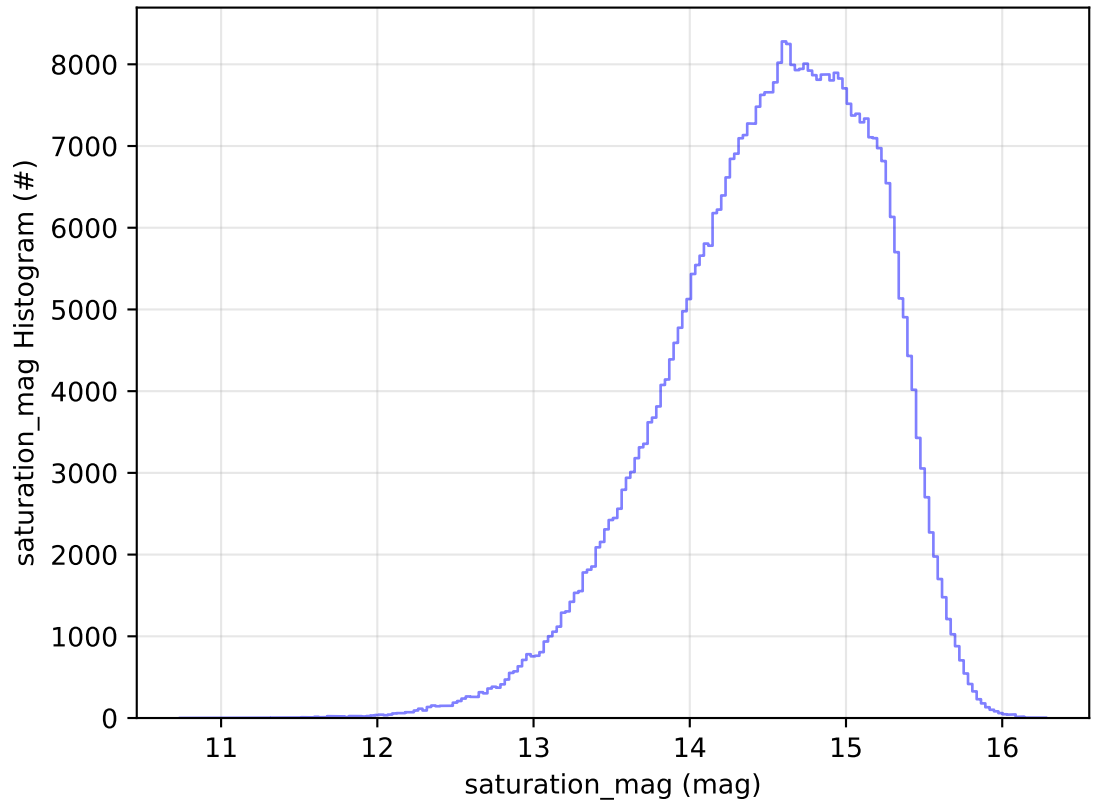
ddf_acor_sf15_lsf20_lsr20_v3.4_10yrs WFD r band: saturation_mag Histogram
