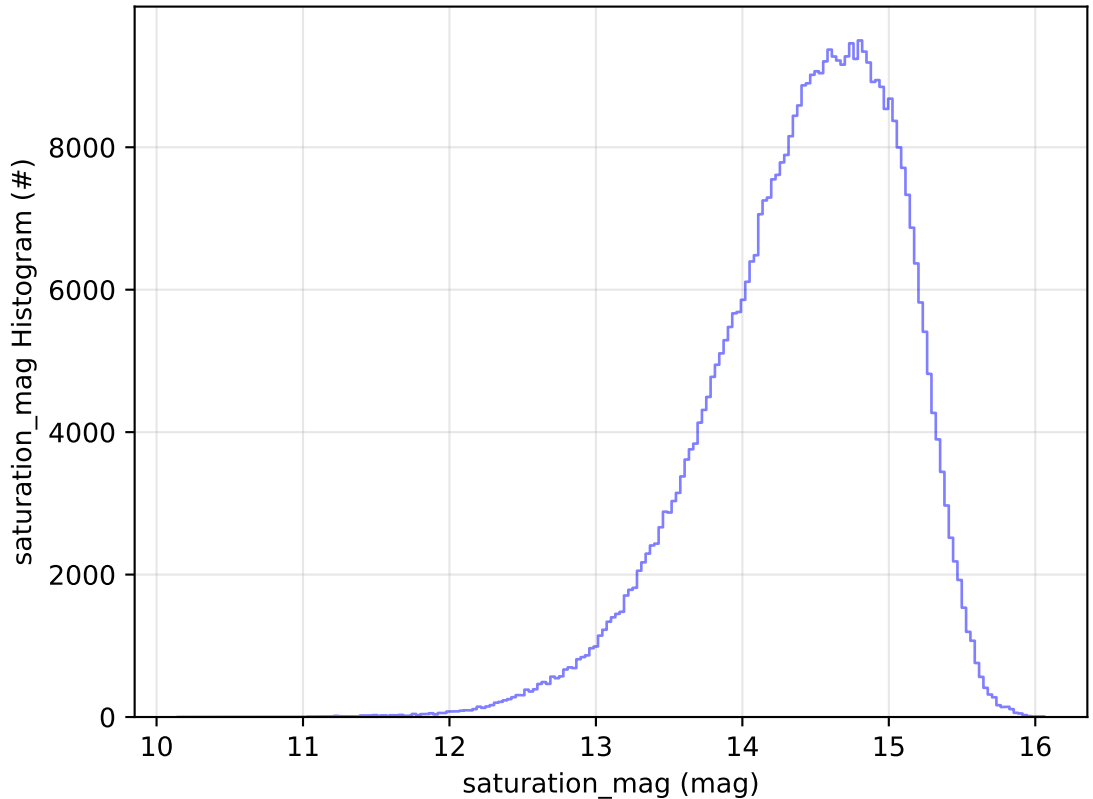
ddf_acor_sf15_lsf20_lsr20_v3.4_10yrs WFD i band: saturation_mag Histogram
