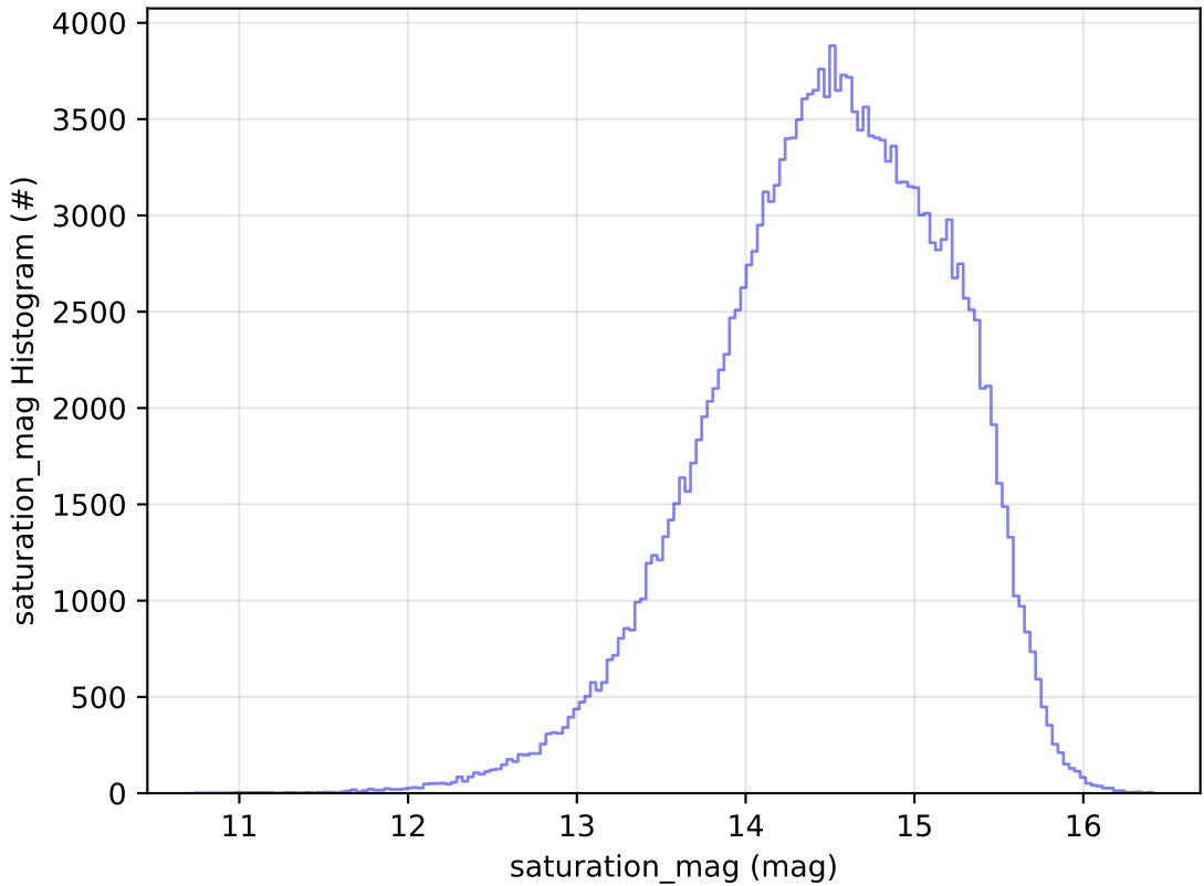
ddf_acor_sf15_lsf20_lsr20_v3.4_10yrs WFD g band: saturation_mag Histogram
