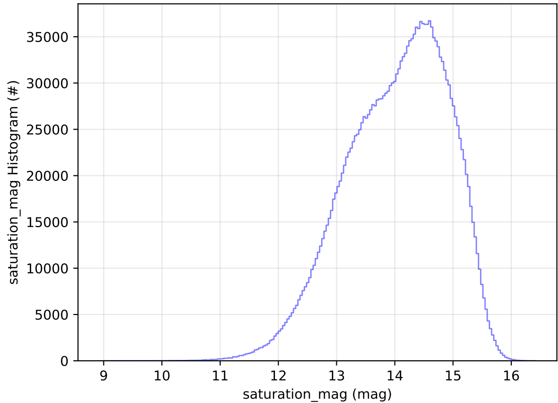
ddf_acor_sf15_lsf20_lsr20_v3.4_10yrs WFD all bands: saturation_mag Histogram
