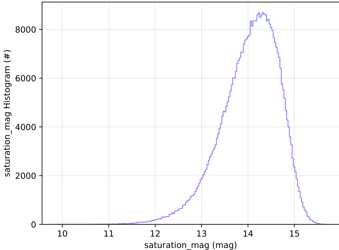
ddf_acor_sf15_lsf20_lsr20_v3.4_10yrs All sky z band: saturation_mag Histogram
