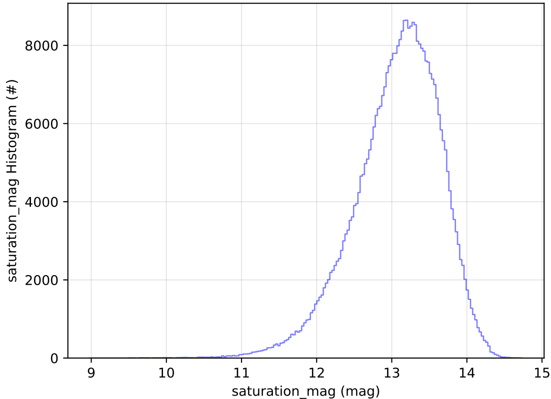
ddf_acor_sf15_lsf20_lsr20_v3.4_10yrs All sky y band: saturation_mag Histogram
