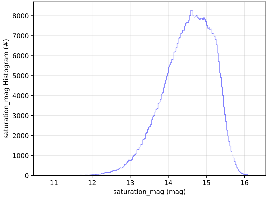
ddf_acor_sf15_lsf20_lsr20_v3.4_10yrs All sky r band: saturation_mag Histogram
