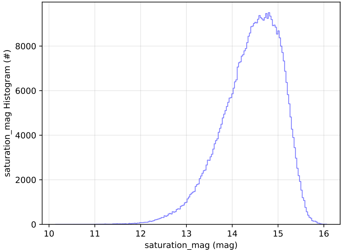
ddf_acor_sf15_lsf20_lsr20_v3.4_10yrs All sky i band: saturation_mag Histogram
