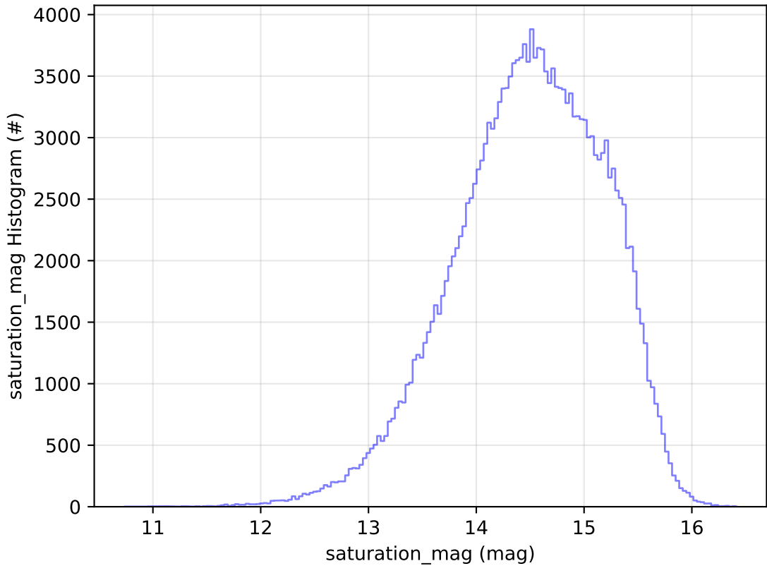
ddf_acor_sf15_lsf20_lsr20_v3.4_10yrs All sky g band: saturation_mag Histogram
