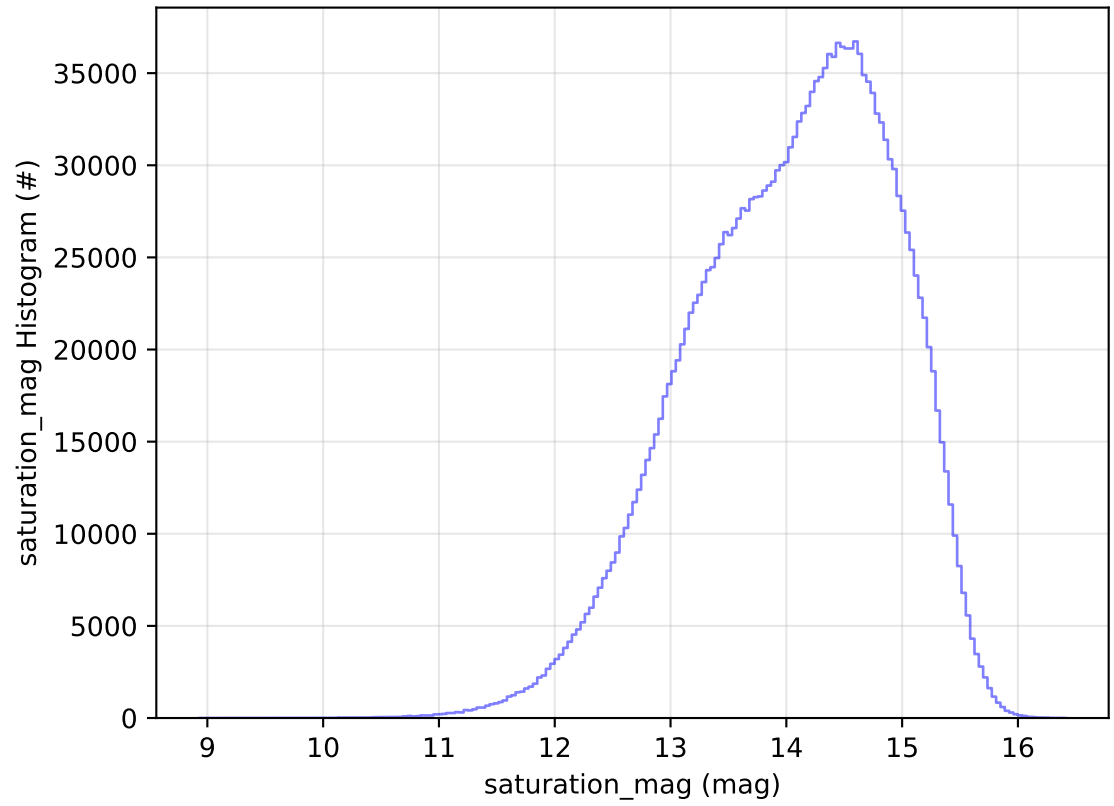
ddf_acor_sf15_lsf20_lsr20_v3.4_10yrs All sky all bands: saturation_mag Histogram
