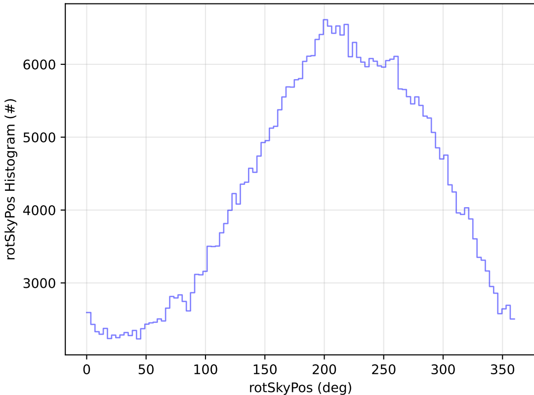
ddf_acor_sf15_lsf20_lsr20_v3.4_10yrs WFD z band: rotSkyPos Histogram
