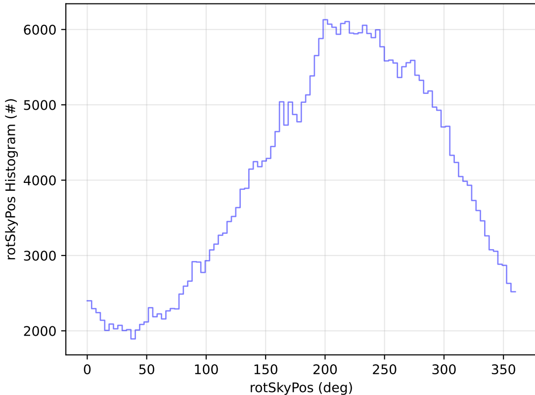
ddf_acor_sf15_lsf20_lsr20_v3.4_10yrs WFD y band: rotSkyPos Histogram
