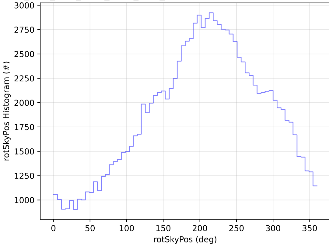
ddf_acor_sf15_lsf20_lsr20_v3.4_10yrs WFD u band: rotSkyPos Histogram
