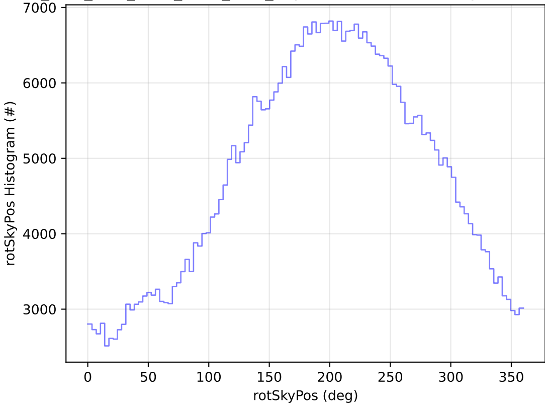
ddf_acor_sf15_lsf20_lsr20_v3.4_10yrs WFD r band: rotSkyPos Histogram
