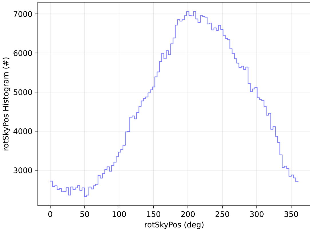
ddf_acor_sf15_lsf20_lsr20_v3.4_10yrs WFD i band: rotSkyPos Histogram
