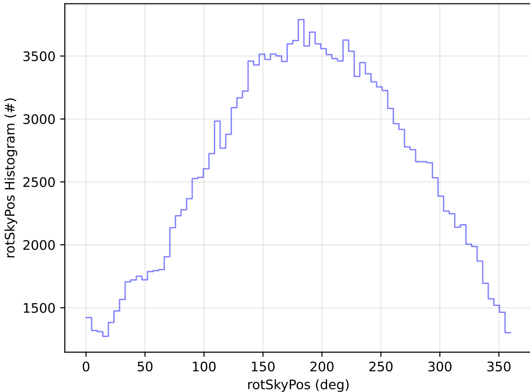
ddf_acor_sf15_lsf20_lsr20_v3.4_10yrs WFD g band: rotSkyPos Histogram
