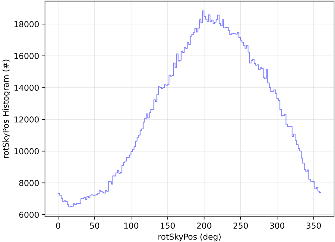
ddf_acor_sf15_lsf20_lsr20_v3.4_10yrs WFD all bands: rotSkyPos Histogram
