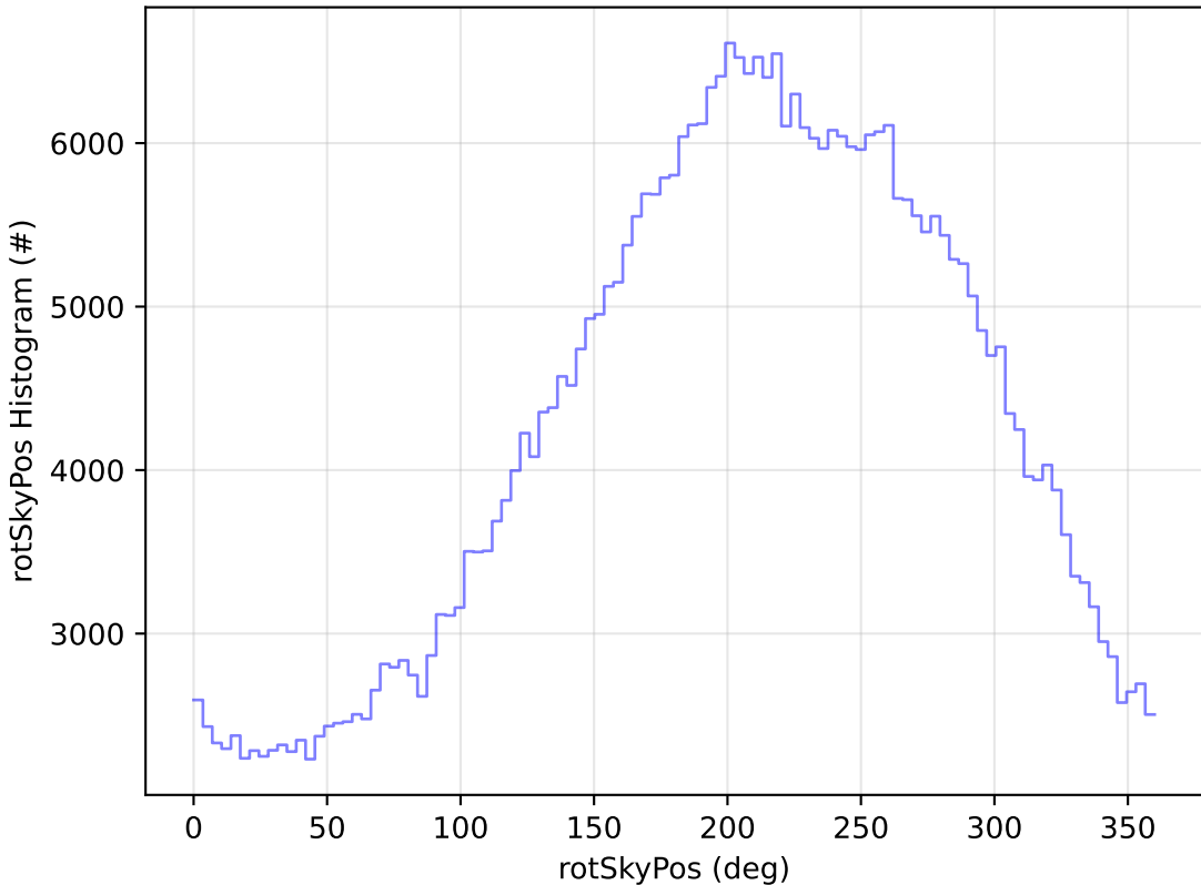
ddf_acor_sf15_lsf20_lsr20_v3.4_10yrs All sky z band: rotSkyPos Histogram
