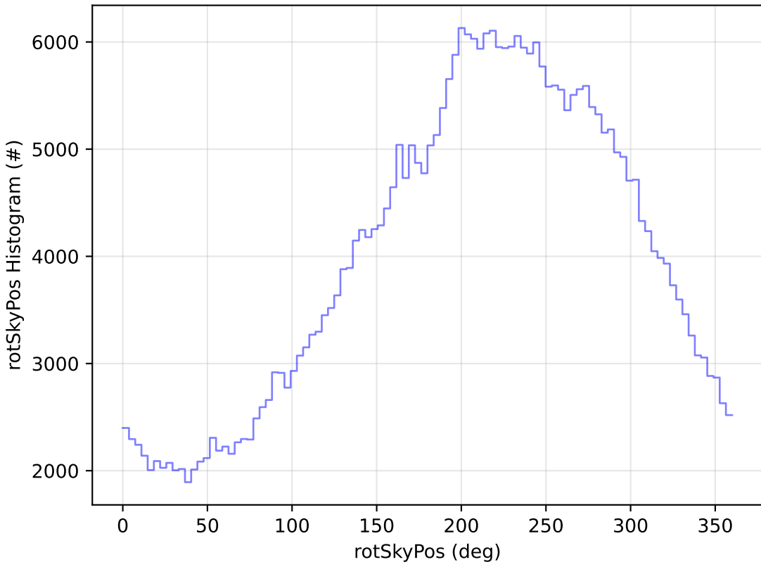
ddf_acor_sf15_lsf20_lsr20_v3.4_10yrs All sky y band: rotSkyPos Histogram
