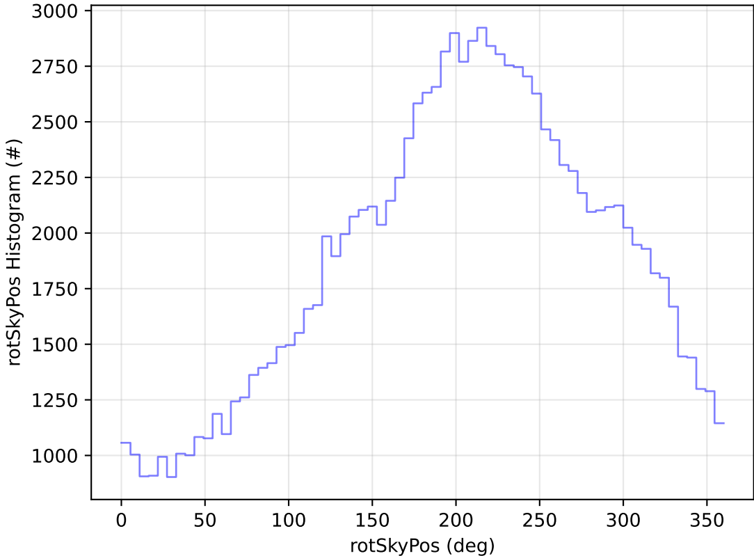
ddf_acor_sf15_lsf20_lsr20_v3.4_10yrs All sky u band: rotSkyPos Histogram
