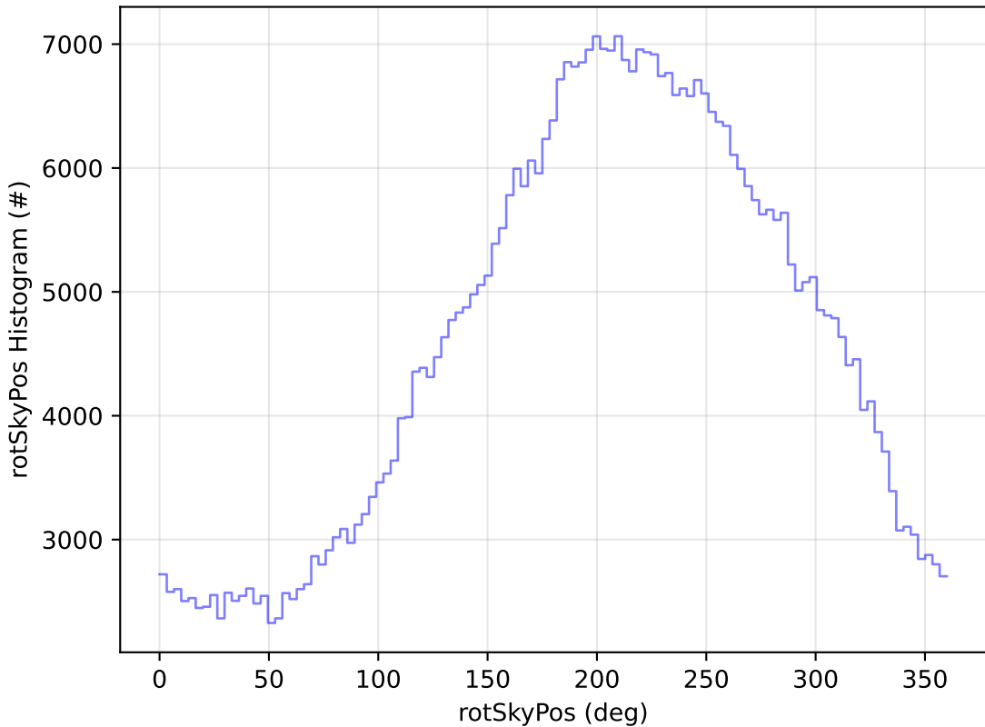
ddf_acor_sf15_lsf20_lsr20_v3.4_10yrs All sky i band: rotSkyPos Histogram
