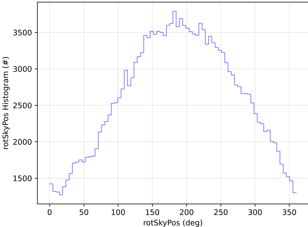
ddf_acor_sf15_lsf20_lsr20_v3.4_10yrs All sky g band: rotSkyPos Histogram
