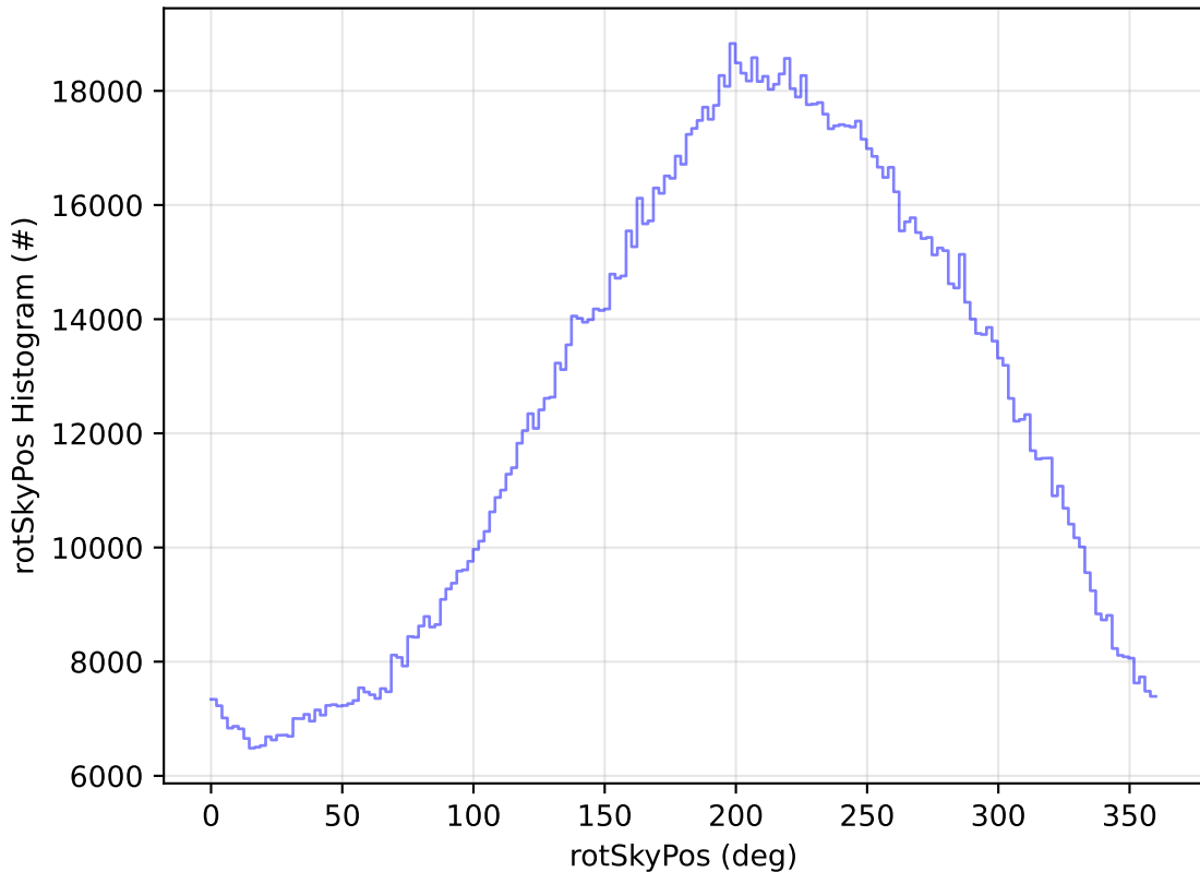
ddf_acor_sf15_lsf20_lsr20_v3.4_10yrs All sky all bands: rotSkyPos Histogram
