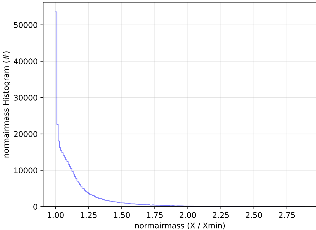
ddf_acor_sf15_lsf20_lsr20_v3.4_10yrs WFD y band: normairmass Histogram
