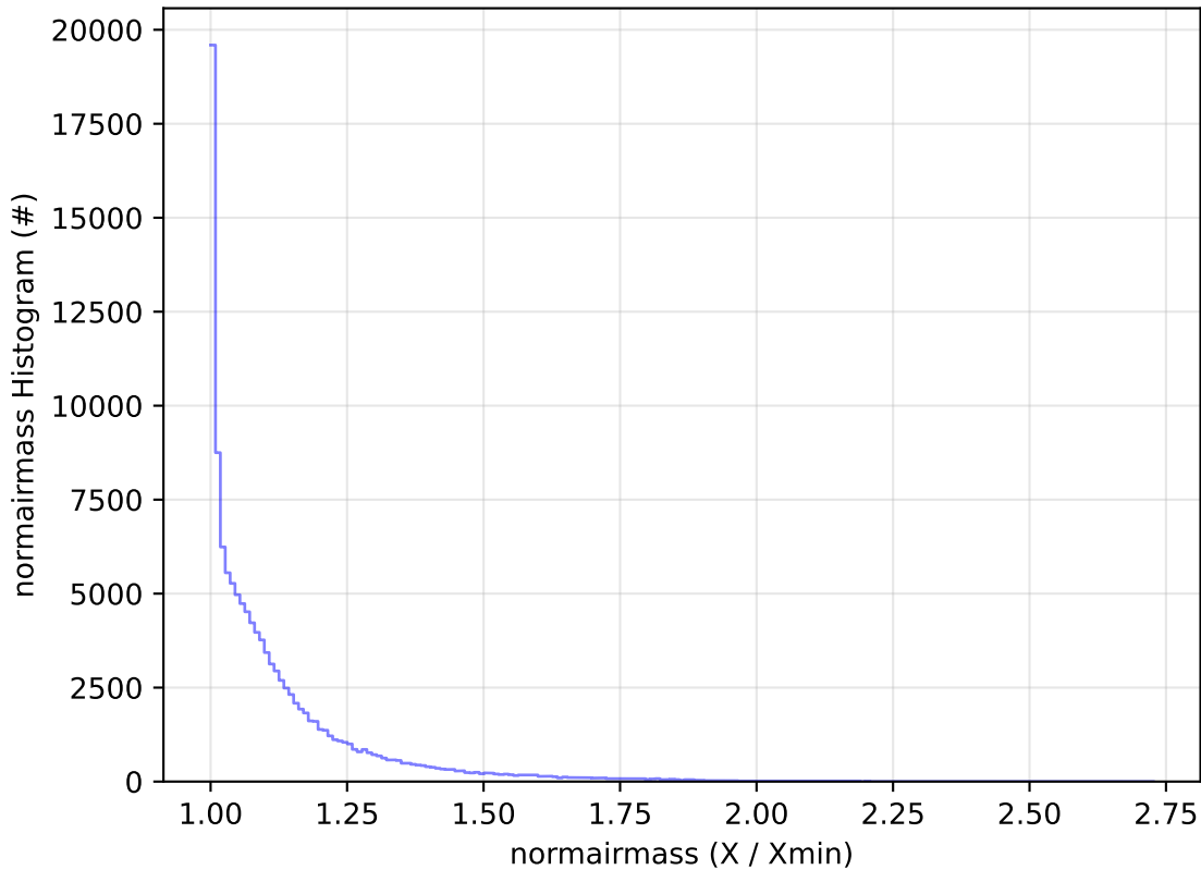
ddf_acor_sf15_lsf20_lsr20_v3.4_10yrs WFD u band: normairmass Histogram
