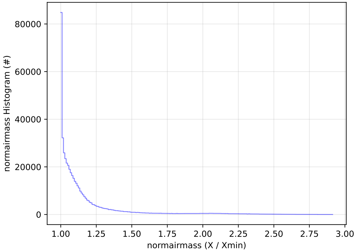
ddf_acor_sf15_lsf20_lsr20_v3.4_10yrs WFD i band: normairmass Histogram
