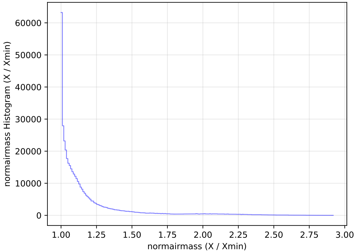
ddf_acor_sf15_lsf20_lsr20_v3.4_10yrs All sky z band: normairmass Histogram
