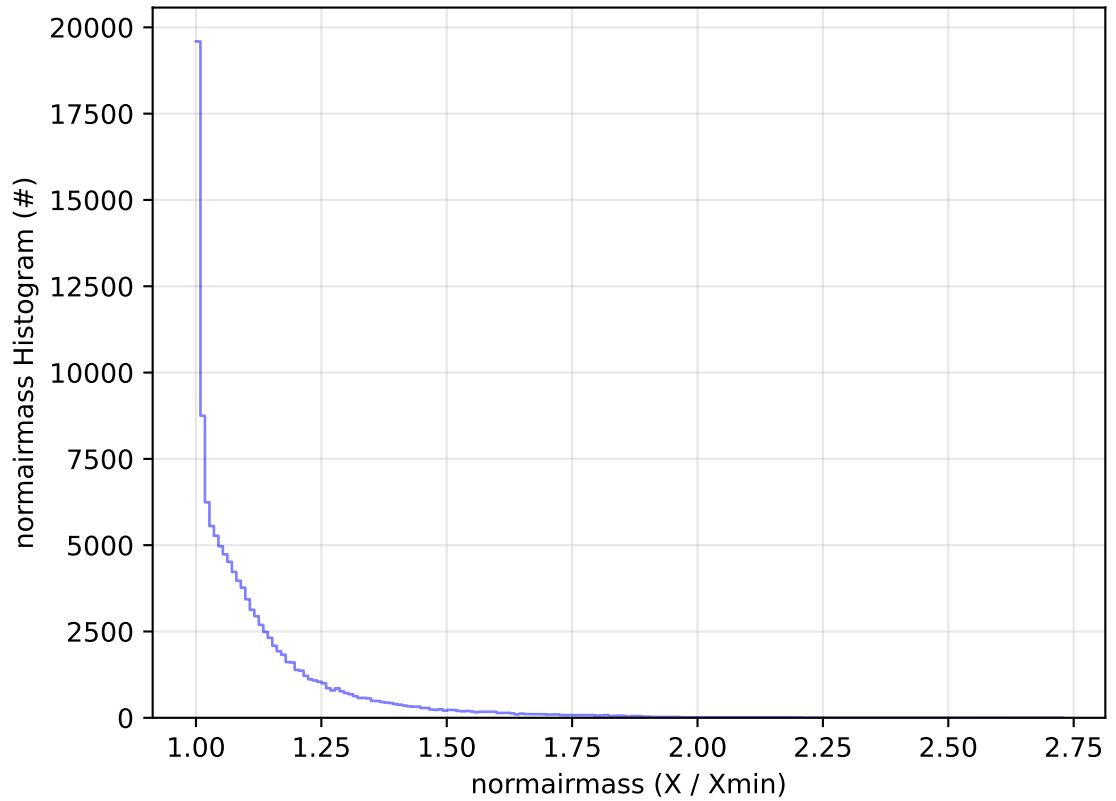
ddf_acor_sf15_lsf20_lsr20_v3.4_10yrs All sky u band: normairmass Histogram
