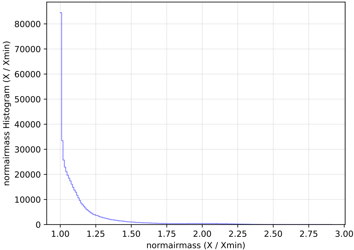
ddf_acor_sf15_lsf20_lsr20_v3.4_10yrs All sky r band: normairmass Histogram
