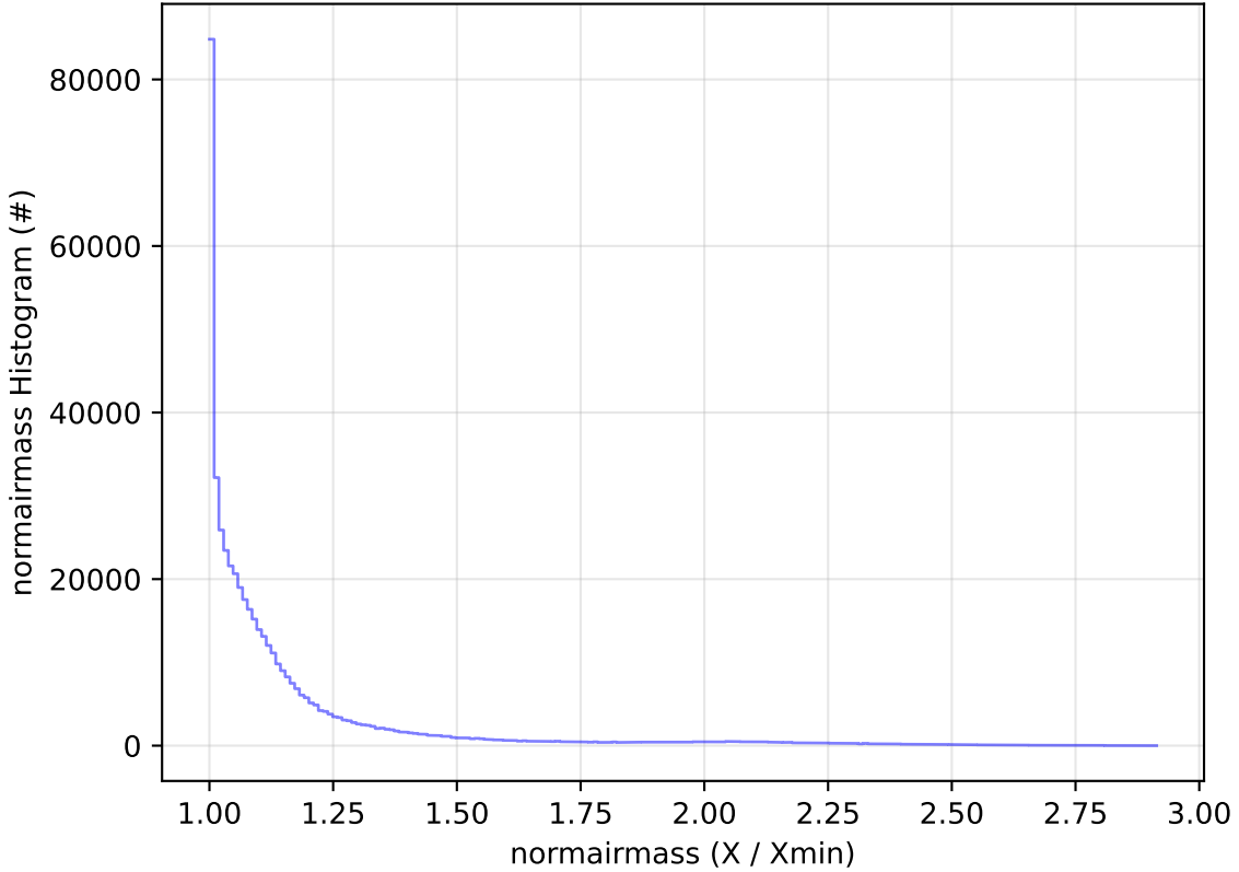
ddf_acor_sf15_lsf20_lsr20_v3.4_10yrs All sky i band: normairmass Histogram
