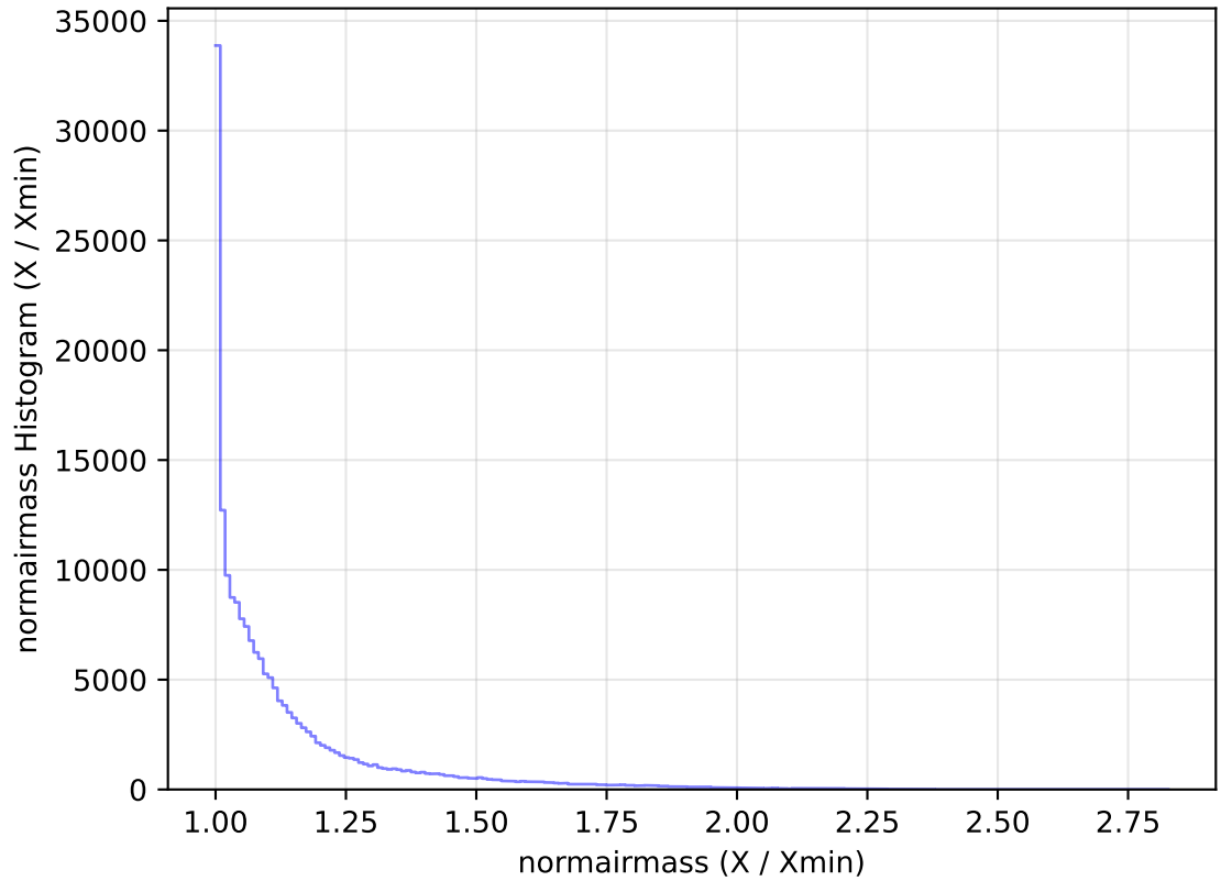
ddf_acor_sf15_lsf20_lsr20_v3.4_10yrs All sky g band: normairmass Histogram
