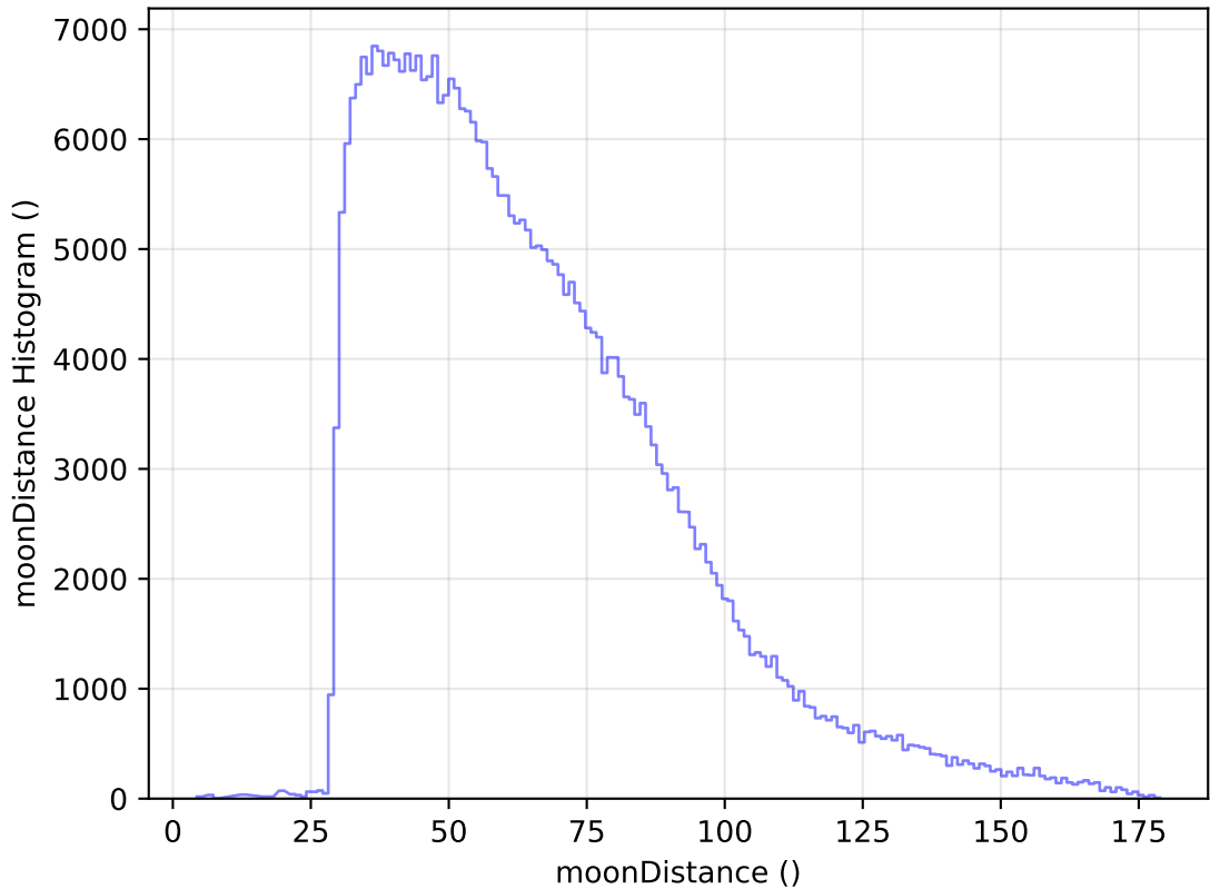
ddf_acor_sf15_lsf20_lsr20_v3.4_10yrs WFD y band: moonDistance Histogram
