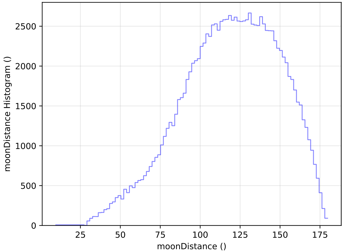
ddf_acor_sf15_lsf20_lsr20_v3.4_10yrs WFD u band: moonDistance Histogram
