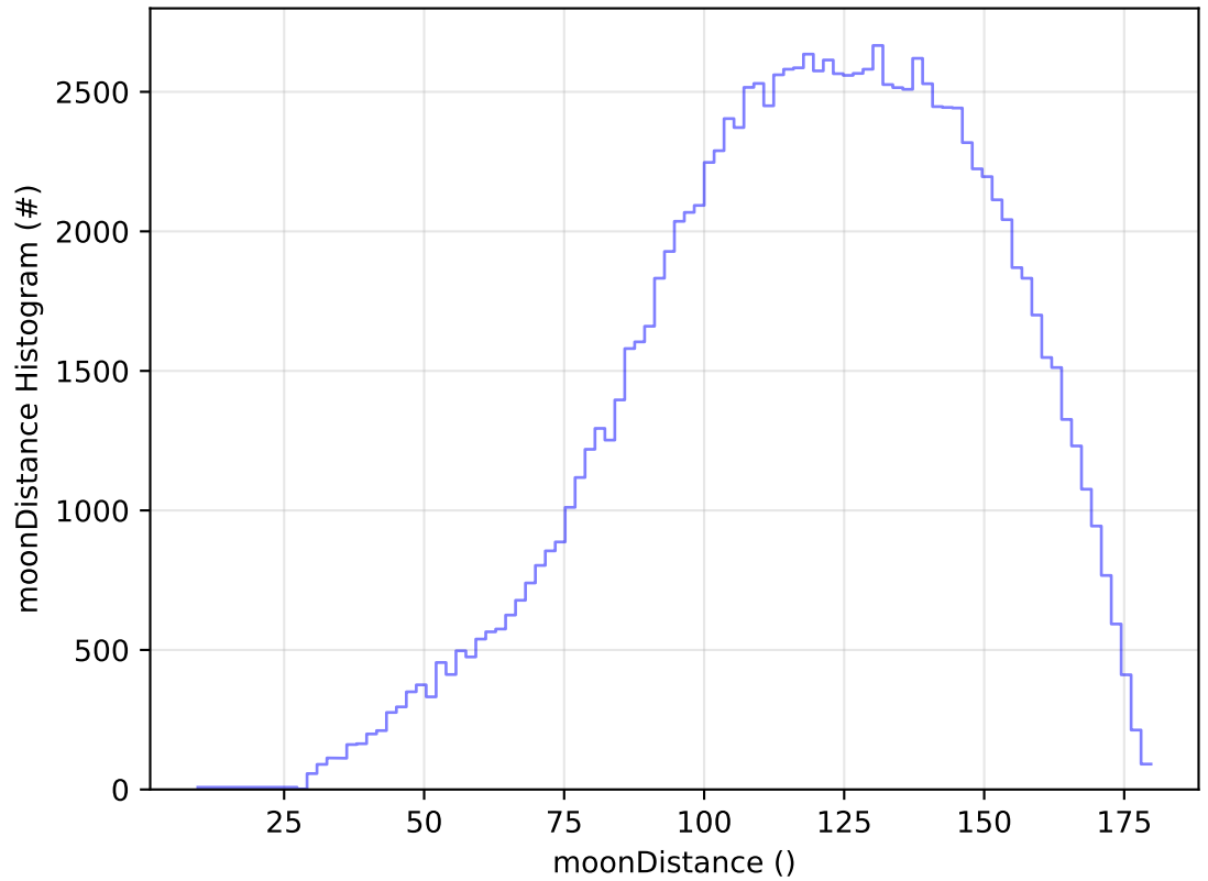
ddf_acor_sf15_lsf20_lsr20_v3.4_10yrs WFD u band: moonDistance Histogram
