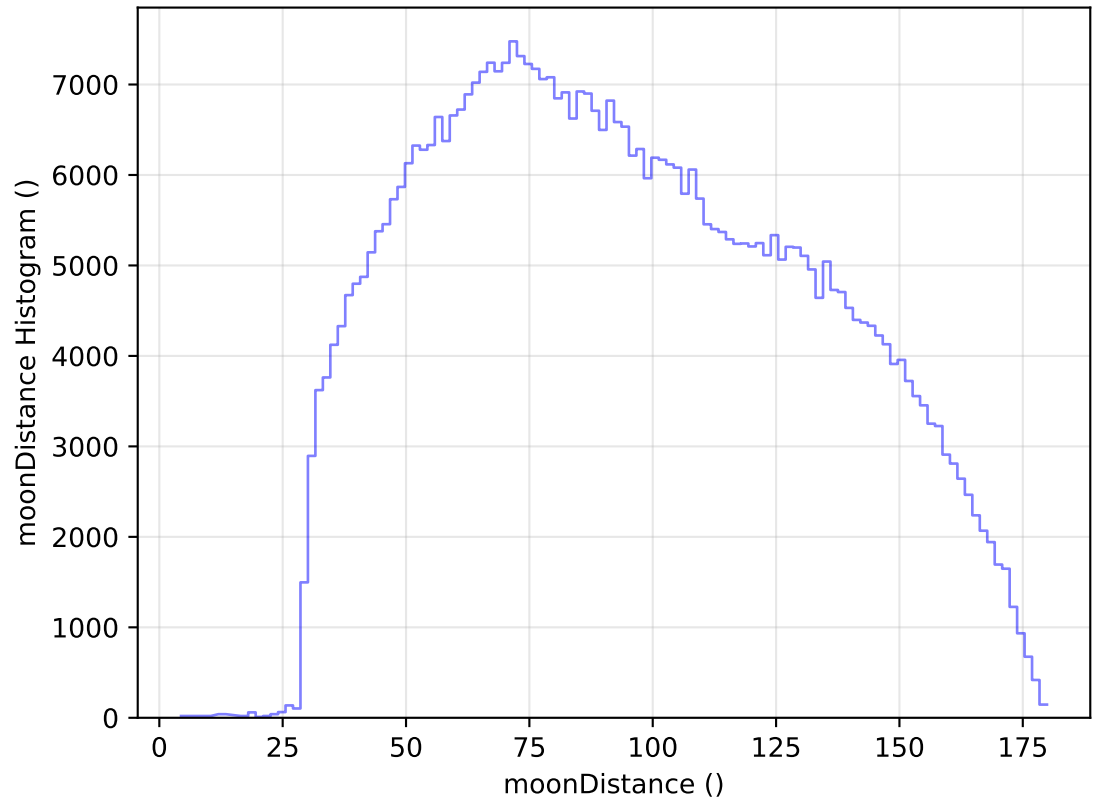
ddf_acor_sf15_lsf20_lsr20_v3.4_10yrs WFD i band: moonDistance Histogram
