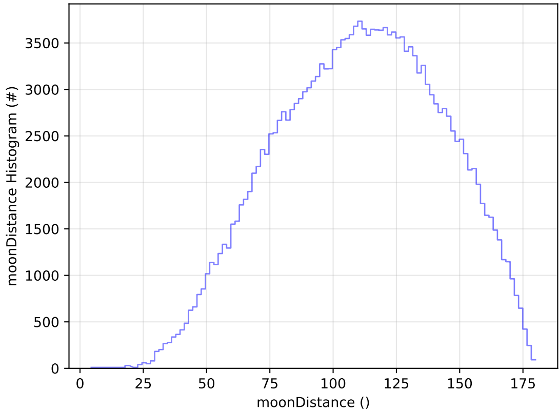
ddf_acor_sf15_lsf20_lsr20_v3.4_10yrs WFD g band: moonDistance Histogram
