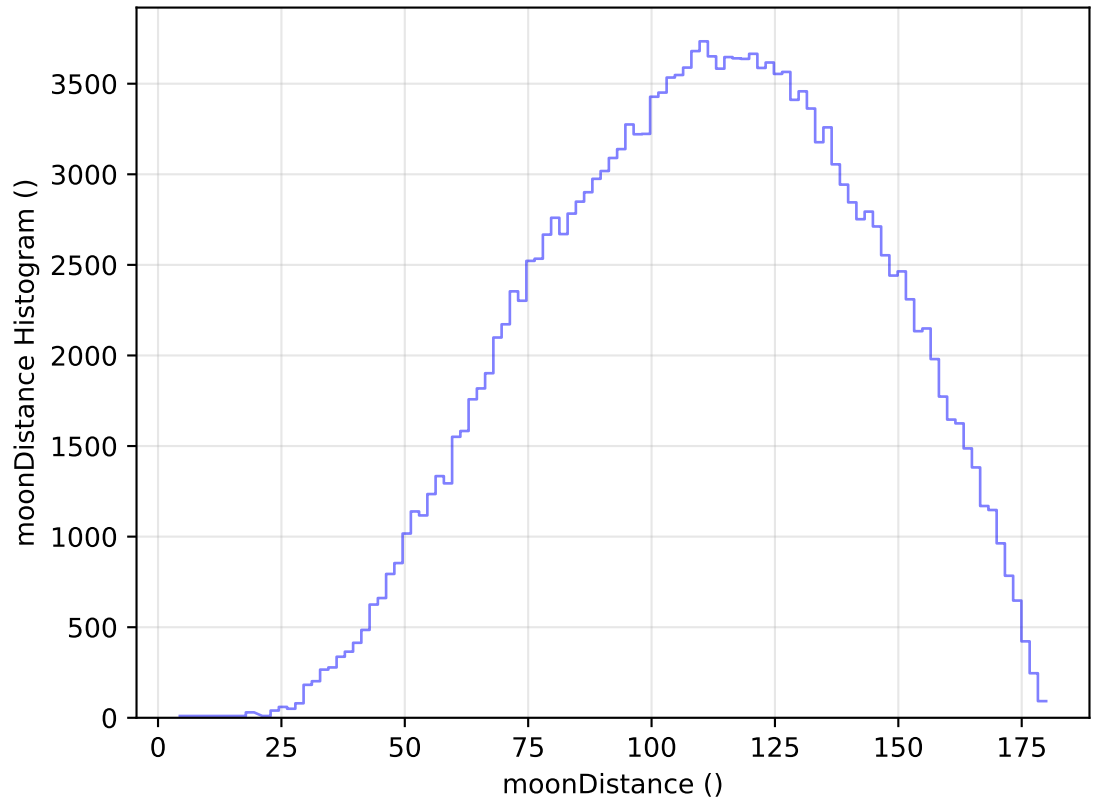
ddf_acor_sf15_lsf20_lsr20_v3.4_10yrs WFD g band: moonDistance Histogram
