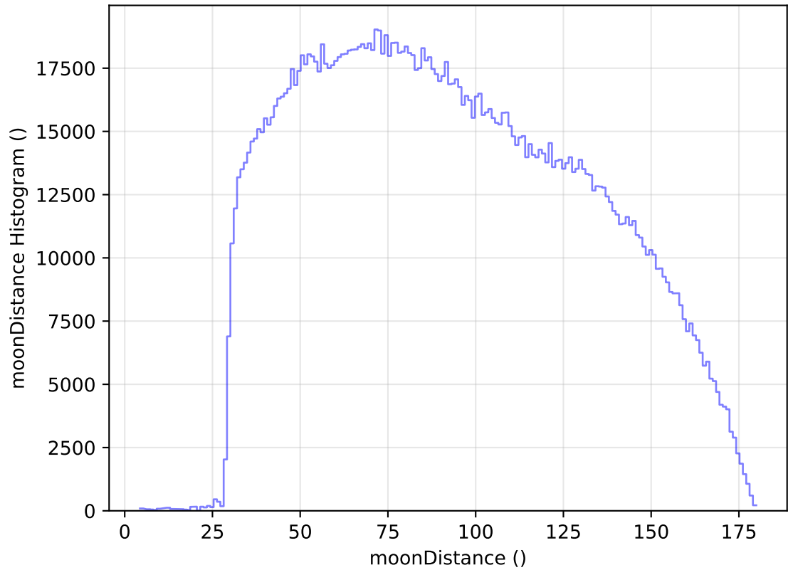
ddf_acor_sf15_lsf20_lsr20_v3.4_10yrs WFD all bands: moonDistance Histogram
