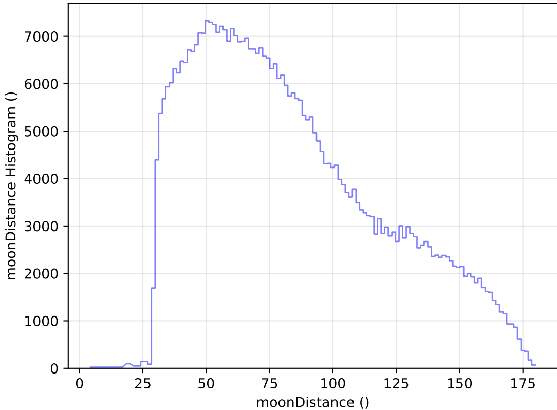
ddf_acor_sf15_lsf20_lsr20_v3.4_10yrs All sky z band: moonDistance Histogram
