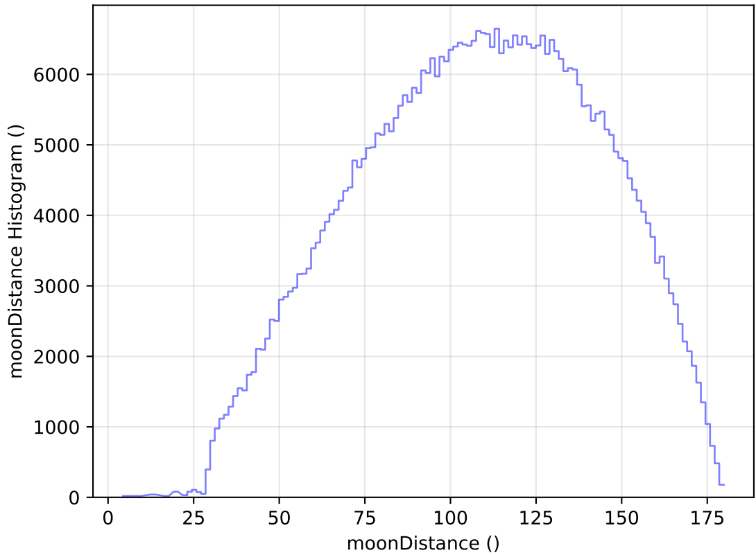
ddf_acor_sf15_lsf20_lsr20_v3.4_10yrs All sky r band: moonDistance Histogram
