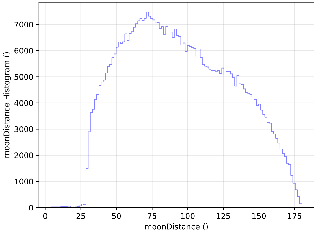
ddf_acor_sf15_lsf20_lsr20_v3.4_10yrs All sky i band: moonDistance Histogram
